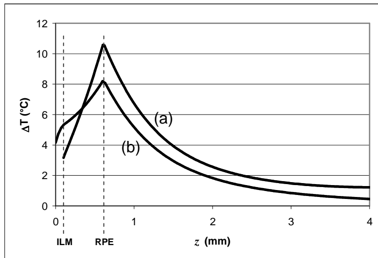
Fig. 6: Temperature rise at t = 60 s, with a spot radius r_s = 1 mm, incident power of 77.5 mW. Curve (a): without ICG. Curve (b): case of a residual ICG-stained vitreous layer of 100 \mu\text{m} overlaying the ILM.
