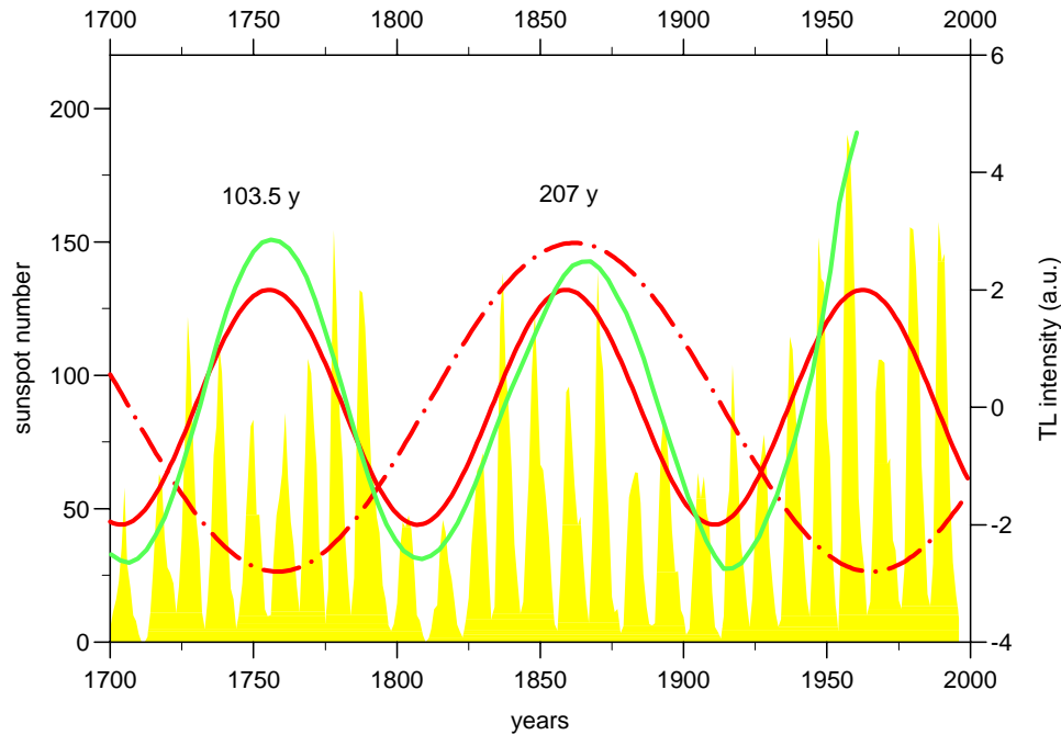
Fig. 3. – 103.5 y and 207 y sinusoidal TL waves (red curves by SE and green curve by SSA) with the sunspot number series (yellow area).
