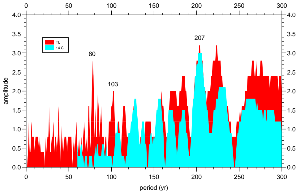
Fig. 2. – Amplitude of the least-square-fit sinusoids to the superposed data as obtained by the method of SE (“stacking”) for the radiocarbon record (blue curve) and for the TL series (red curve) as a function of period T .
