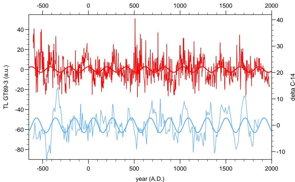
Fig. 1. - The red curve shows the TL time series of the GT89-3 core, detrended by SSA (PCs 1-2) and the blue curve the \Delta^{14}\text{C} decadal tree ring record [7]. Superposed to the data are shown the 207 y waves, estimated by the method of SE.
