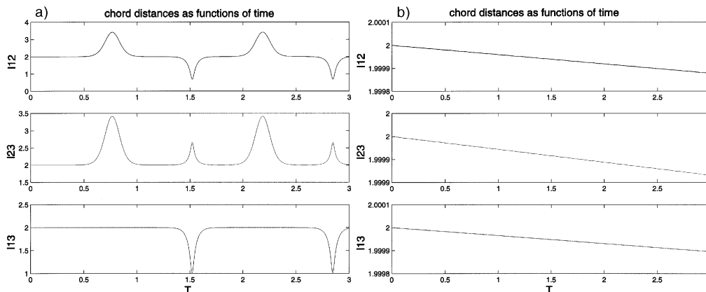
Fig. 2. – Chord distances as functions of time. Equilateral triangle relative equilibrium. a) Unstable, \Gamma_1 = 2, \Gamma_2 = 1, \Gamma_3 = -2, \det \delta^2 H_\xi = -4 . b) Stable, \Gamma_1 = 2, \Gamma_2 = 1, \Gamma_3 = 4, \det \delta^2 H_\xi = 14 .
