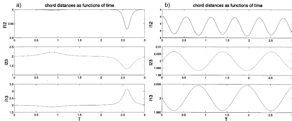
Fig. 1. – Chord distances as functions of time. Great circle relative equilibrium. a) Unstable, \Gamma_1 = 3, \Gamma_2 = 2, \Gamma_3 = 0.2, \det \delta^2 H_\xi = -1 . b) Stable, \Gamma_1 = 3, \Gamma_2 = 2, \Gamma_3 = 0.02, \det \delta^2 H_\xi = 0.8 .
