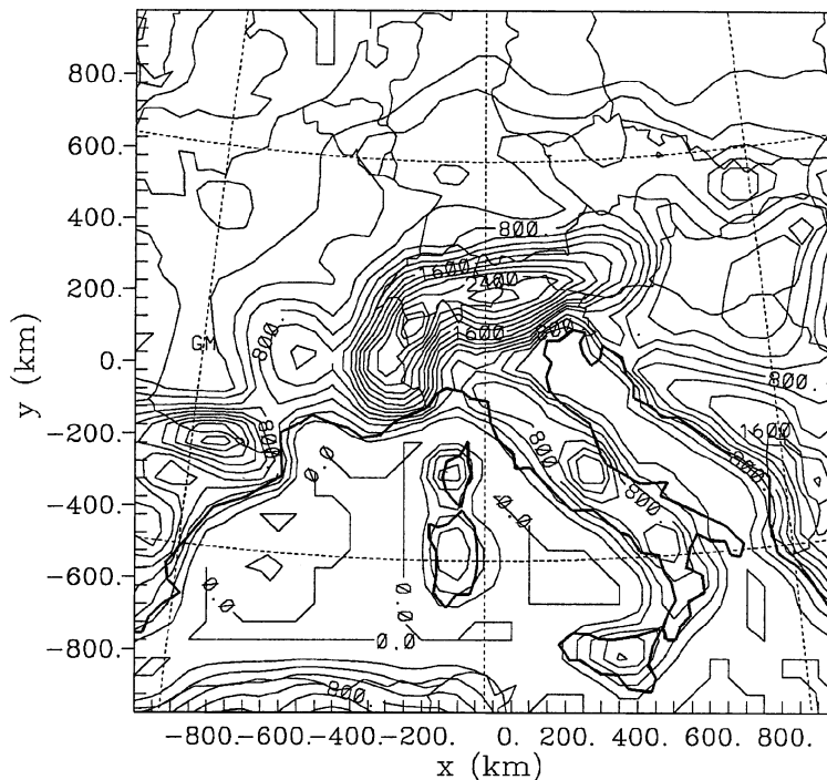
Fig. 1. – Topography of simulation domain (m).
