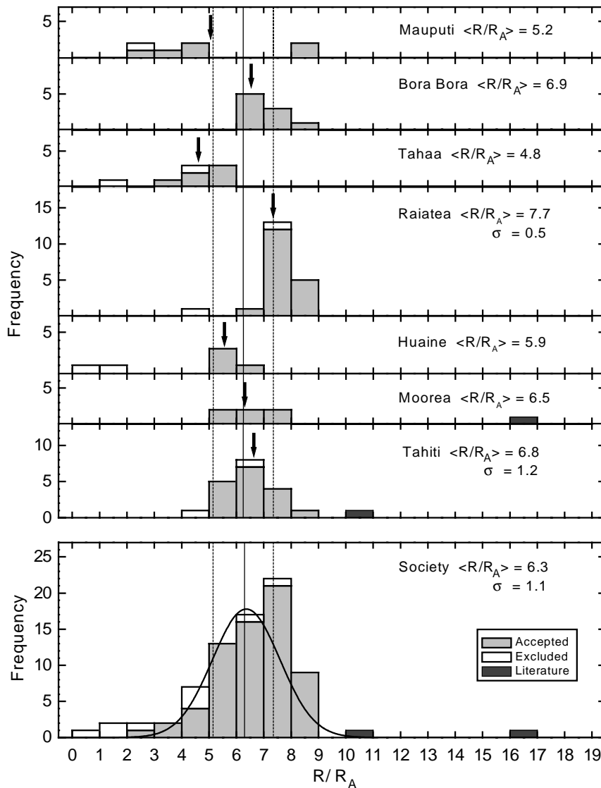
Fig. 3. – Frequency of ^3\text{He}/^4\text{He} in basalt samples for islands of the Society chain. The isotopic ratio is expressed in unit R_A of the ^3\text{He}/^4\text{He} in atmosphere ( R_A = 1.4 \times 10^{-6} ). All values from this work, except those marked with a black box coming from Hanyu and Kaneoka, 1992. Values marked with a white box are samples with blank > 10\% and/or helium concentration lower than 0.5 \text{ ncc/g} . The curve represents the Gaussian with \langle R/R_A \rangle = 6.3 (solid line along the figure) and \sigma = 1.1 (dashed lines). The arrows represent the mean value for each island.
