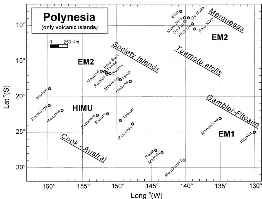
Fig. 1. – The Polynesian region. The fracture zone locations are taken from Dupuis et al. , 1989 and Hemond et al. , 1994. The indicative identifications EM1, EM2, HIMU are taken from [1] and [7].
