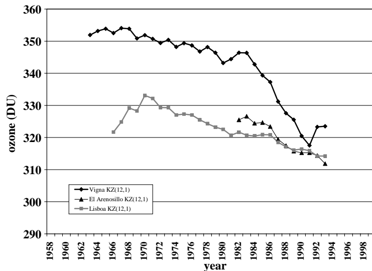
Fig. 2. – Winter series by using the KZ(12,1). Diamond marker line for Vigna di Valle series, grey square marker line for the Lisbon one and triangle marker line for that of El Arenosillo station.
