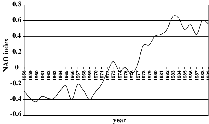
Fig. 3. – NAO Index time series.
