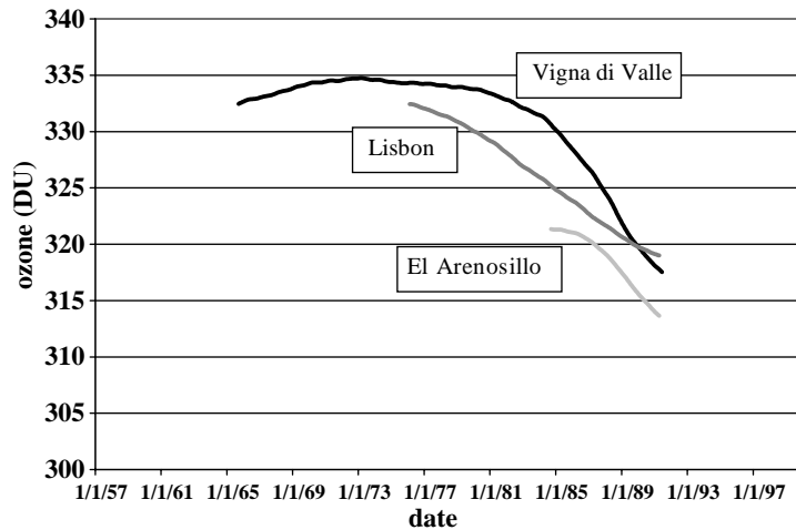
Fig. 1. – Filtered series by using the KZ(105,2).
