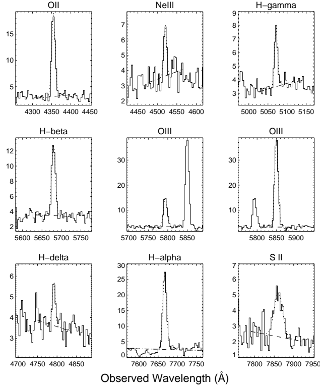
Fig. 1. – The figure shows the nine lines detected in our VLT spectrum. The vertical axes represent the flux densities in units of 10^{-18} \text{ erg s}^{-1} \text{ cm}^{-2} \text{ \AA}^{-1} . The values of the lines' integrated fluxes can be seen in [16].
