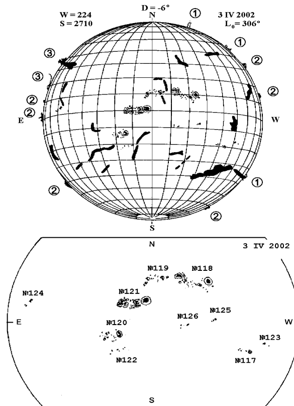
Fig. 2. – The heliographic map of magnetic fields and active regions of the Sun for 3 April 2002. Near the center (to the left and above) there is an oval dark nucleus of AR No. 121. Active regions are contoured by dotted lines. Dark oblong formations are relatively cold filaments. Below is given an enlarged central part of the disk with AR numbers. Wavy lines round the Sun show magnitudes of corona brightness (in relative units). To the left and above are given total parameters of sunspots: Wolf number W = 224 and spots' area S = 2710 mph. The area of AR No. 121 S = 390 mph was at a maximum on 3 April 2002 (mph—millionth parts of hemisphere).
