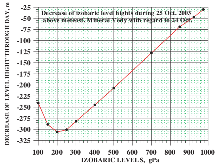
Fig. 8. – A decrease of isobaric levels from the data of radiowave sounding over the meteorological station Mineral Vody on 24-25 October 2003. Extrapolation of the decreasing trend above 100 hPa level indicates that even above 100 hPa level the decrease constituted not less than 150 \text{ m day}^{-1} . The latter fact is an additional confirmation of uniformity of the increase in the air column over the region of sounding as a whole. Apparently, this could take place only under the influence of an external forcing factor.
