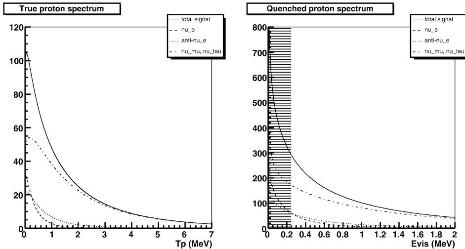
Fig. 4. – Left: the theoretical proton spectrum in Borexino, from \nu - p elastic scattering; the contributions from \nu_e , \bar{\nu}_e and the sum of \nu_\mu , \nu_\tau , \bar{\nu}_\mu and \bar{\nu}_\tau are shown with dotted or dashed lines; the solid line is the sum spectrum for all flavors. Right: the same spectrum, with the quenching effect taken into account (the dotted region represents the energy range suppressed by the solar neutrino threshold at 250 keV).
