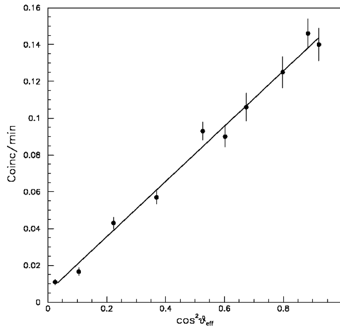
Fig. 5. – Angular distribution of cosmic rays, measured by a telescope of two small Geiger counters, placed 10 cm apart. Data are reported as a function of \cos^2 \theta to show their approximate linear trend. Solid line is a weighted fit to the data.
