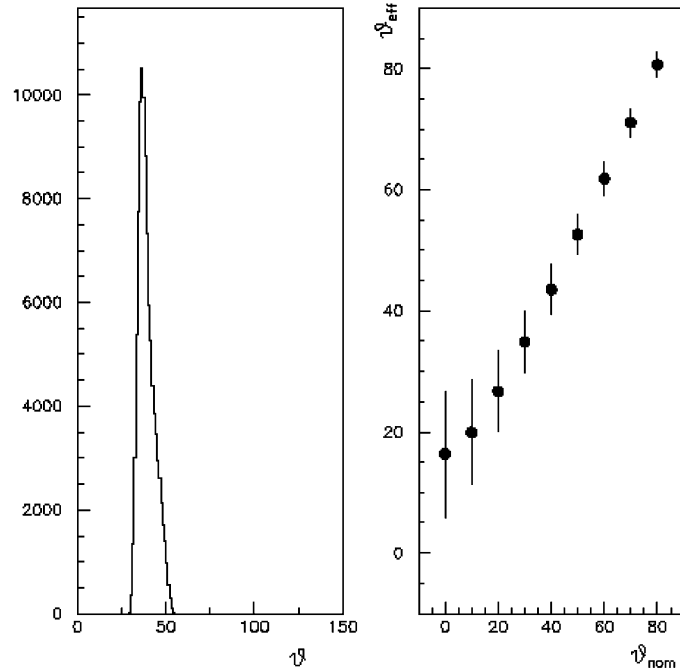
Fig. 6. – Left: distribution of the polar angles for cosemics traversing two Geiger counters of finite size, placed 10 cm apart, at a nominal angle \theta = 40^\circ . Right: effective angle subtended by two Geiger counters, as a function of the nominal angle of the telescope.
