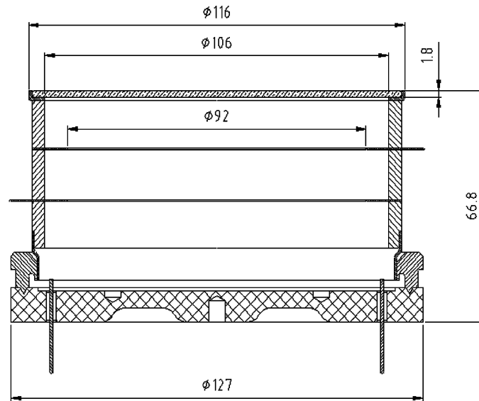
Fig. 4. – Cross-section of the proximity focused prototype HPD.
