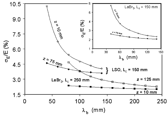
Fig. 17. – Dependence of the statistical term of the energy resolution ( E = 511 keV) on the bulk absorption length of the scintillator crystal.
