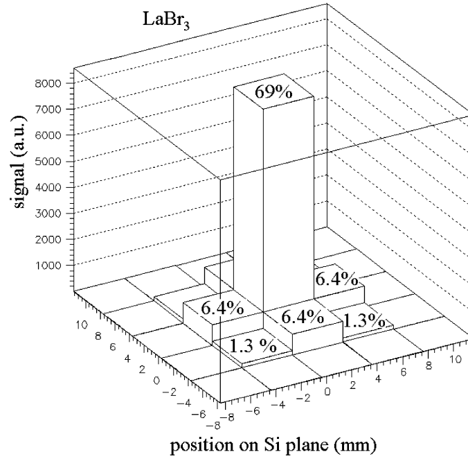
Fig. 15. – Simulated distribution of the hit map on the silicon sensor for the readout of a scintillator crystal centred over the central Si pad.
