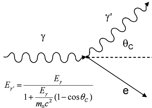
Fig. 27. – Kinematics of the Compton interaction.
