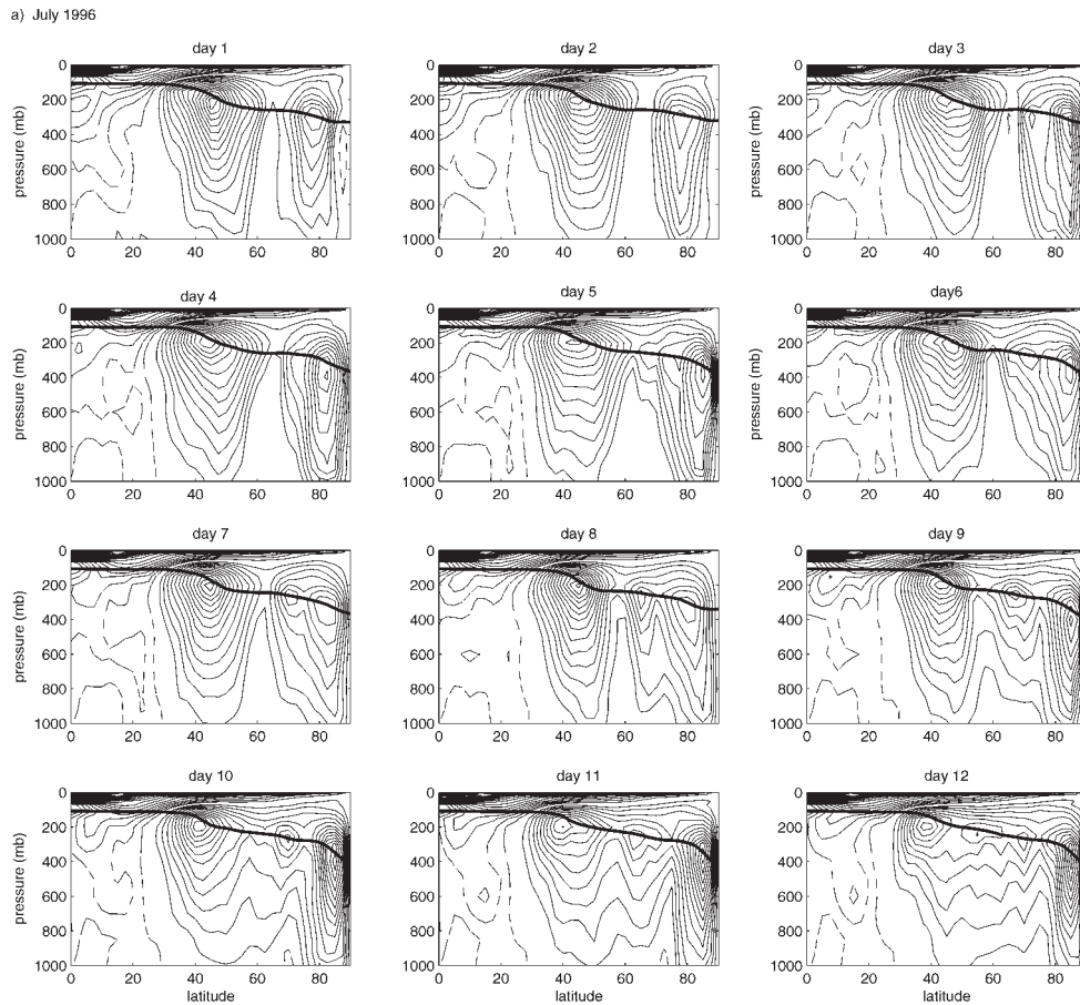
Fig. 3. – Latitude-height (pressure) cross-section of daily zonal mean zonal wind for: a)–b) July 1996 days 1–12, 25–31, and c) July 1985 days 10–21. Contour interval is 2 \text{ ms}^{-1} and zero line is excluded; dashed lines denote negative values and thick line marks the tropopause pressure.
