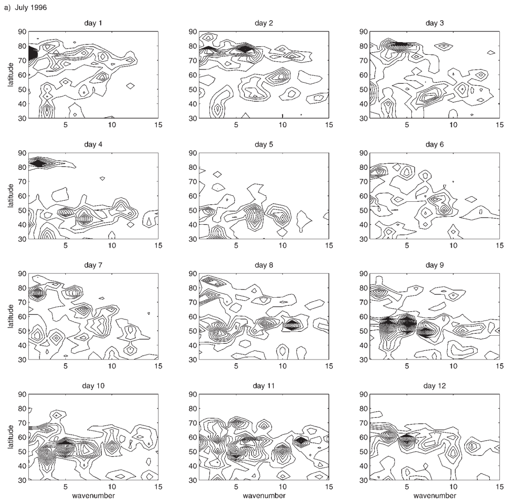
Fig. 5. – Daily power spectra of the meridional eddy heat fluxes ( v'T' ) at 850 mb as a function of the zonal wave number and latitude: a)–b) July 1996 days 1–12, 25–31, and c) July 1985 days 10–21. Unit is \text{m}^2 \text{s}^{-2} \text{K}^2 , contour interval is 2 \times 10^3 \text{m}^2 \text{s}^{-2} \text{K}^2 and zero line is excluded.
