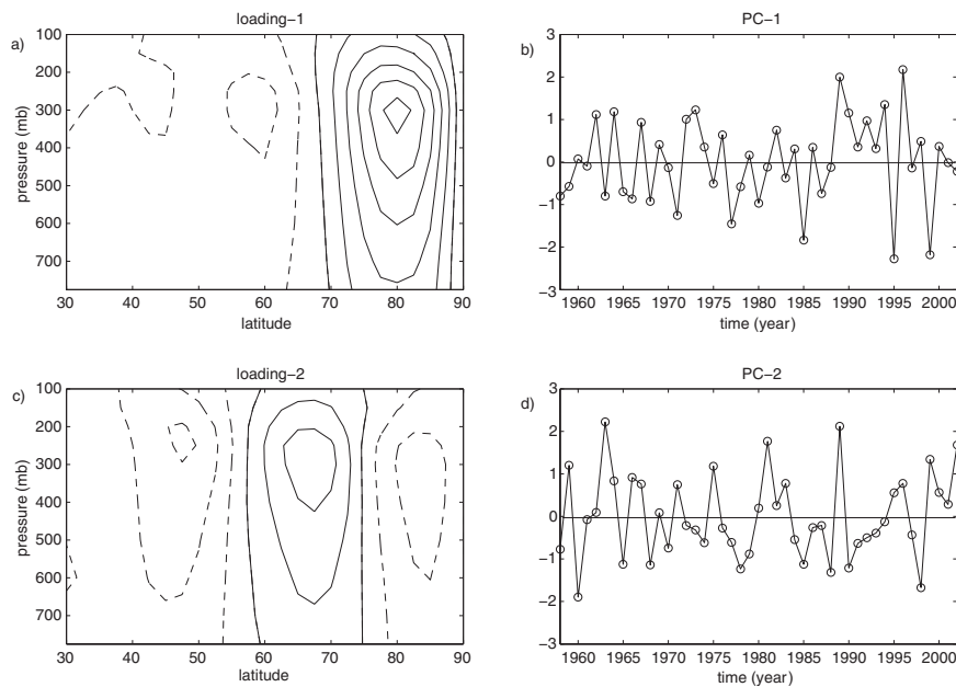
Fig. 7. – PCA: First two loadings and corresponding standardized PC scores of the zonal mean zonal wind for July from 100 mb down to 775 mb and in the latitude band 30°N–90°N. Unit in a) and c) is \text{ms}^{-1} ; contour interval is 0.5 \text{ ms}^{-1} , zero line is excluded and dashed lines denote negative values.
