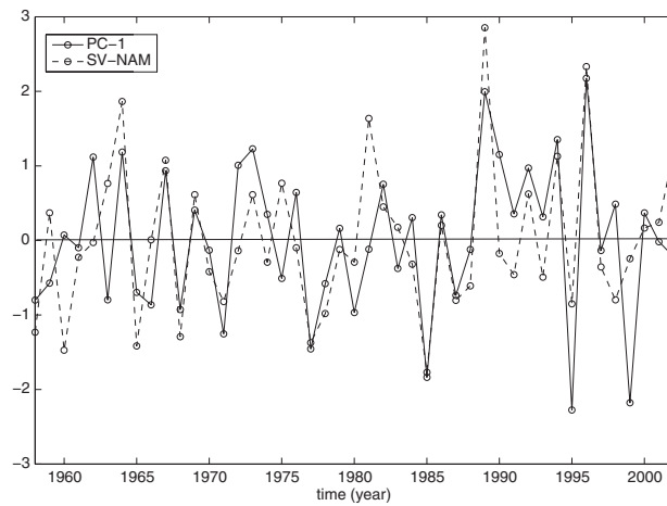
Fig. 9. – Time behaviour of PC-1 shown in fig. 7b (solid line) and the NAM index (dashed line). Data are ERA-40 from 1958 to 2002.
