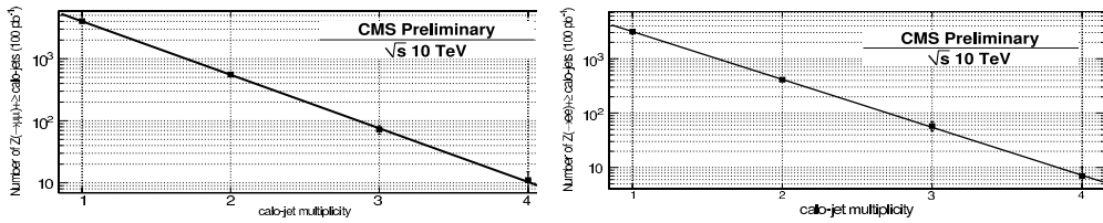
Fig. 2. – The (dN/dn_{\text{jet}}) distributions and exponential fit for Z(\rightarrow \mu\mu) + \text{calo-jets} (left) and Z(\rightarrow ee) (right).
