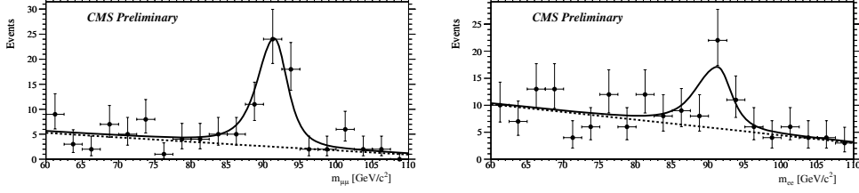
Fig. 1. – Invariant mass m(\mu\mu) (left) and m(ee) (right) for Z + \geq 4 track-jets events selected in a simulated sample equivalent to 100 \text{ pb}^{-1} .
