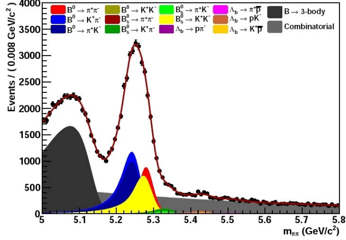
Fig. 2. – Distribution of the B \rightarrow h^+ h^- invariant mass from a Monte Carlo sample corresponding to an integrated luminosity of 0.2 \text{ fb}^{-1} , with the result of the maximum likelihood fit superimposed. The various signal and background components contributing to the whole line shape are also shown.
