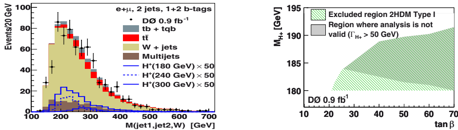
Fig. 4. – Left: D0 distribution of the discriminating variable M(\text{jet1}, \text{jet2}, W) for the data and the expected signal and backgrounds. Right: exclusion region in the \tan\beta - M_{H^\pm} space.
