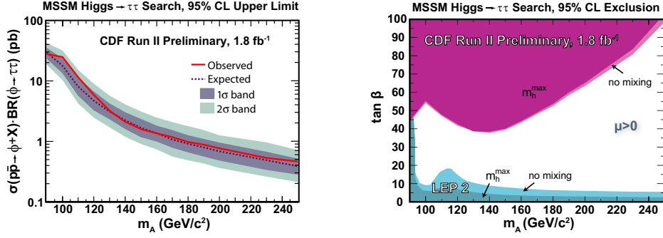
Fig. 1. – Left: CDF cross-section upper limit for the process \Phi \rightarrow \tau^+\tau^- , as a function of M_A . Right: corresponding exclusion region at 95% CL in the plane m_A - \tan\beta , for the maximum Higgs mass and the no-mixing scenarios, with the Higgs mixing parameter \mu \geq 0 .
