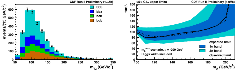
Fig. 2. – Left: the CDF mass distribution of two leading jets in events with three b-tagged jets, for the b\Phi \rightarrow bbb search. Right: 95% CL exclusion region in the m_A - \tan\beta space.
