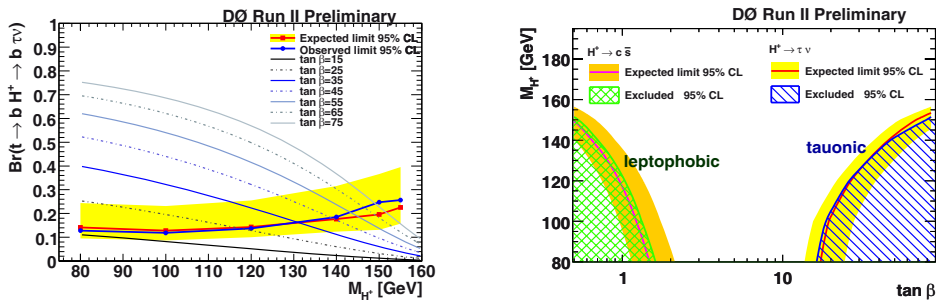
Fig. 3. – Left: D0 cross-section upper limit for the t \rightarrow bH^+ \rightarrow b\tau^+\nu process, as a function of M_{H^\pm} . Right D0 exclusion regions at 95% CL in the plane \tan\beta - M_{H^\pm} for the decay in the leptophobic ( H^+ \rightarrow c\bar{s} ) and tauonic ( H^+ \rightarrow \tau^+\nu ) scenarios.
