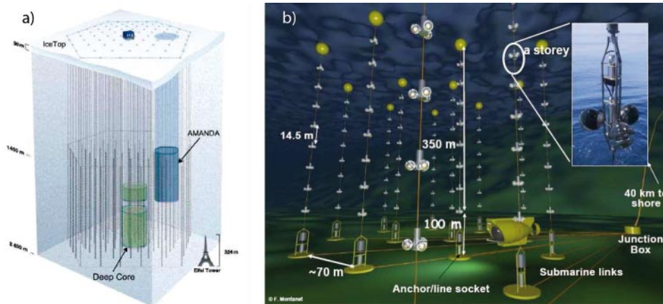
Fig. 2. – (a) The IceCube detector side view, with the AMANDA detector as a part in the right. Currently there are 59 buried InIce strings. The IceTop surface array and the DeepCore are also shown. (b) Schematic view of the ANTARES detector, completed in May 2008.
