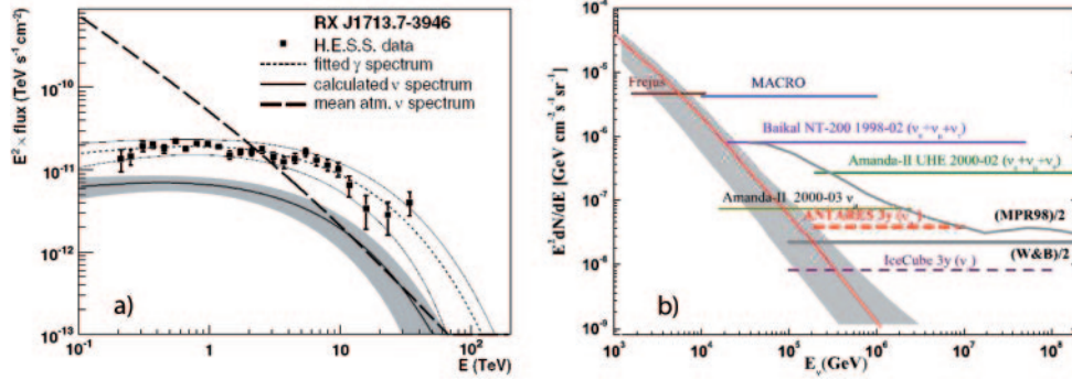
Fig. 1. – (a) Measured gamma-ray flux from the shell-type supernova RX J1713.7-3946 and estimated neutrino flux [3] with their error bands. (b) Sensitivities and upper limits for a E^{-2} diffuse HE neutrino flux. Experimental upper limits are indicated as solid lines, the ANTARES and IceCube 90% CL sensitivities with dashed lines. For reference, the W&B and MPR98 limits for transparent sources are also shown. Part of the MPR98 upper bound is already excluded by the AMANDA-II result.
