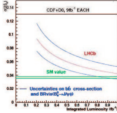
Fig. 4. – (Colour online) Statistical uncertainty on \phi_{J/\psi\phi} vs. the integrated luminosity. The blue lines show the uncertainties coming from the b\bar{b} cross-section and the visible branching ratio on B_s^0 \rightarrow J/\psi\phi . The green band is the SM value. The Tevatron line is the combined CDF/D0 uncertainty in 2008 scaled to 18\text{fb}^{-1} , as expected by the end of run 2.
