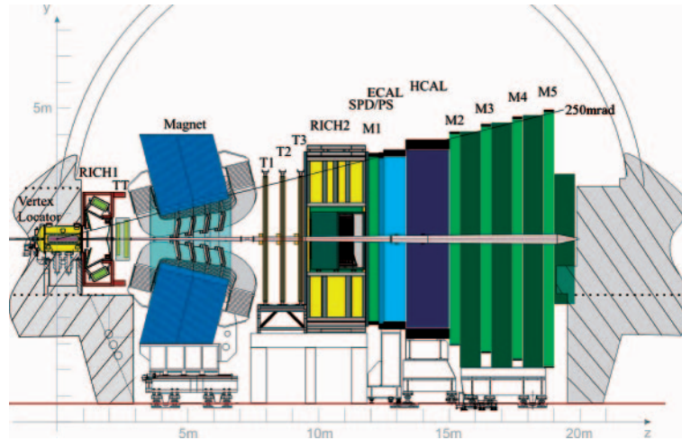
Fig. 2. – Side view of the LHCb detector showing the Vertex Locator (VELO), the dipole magnet, the two RICH detectors, the four tracking stations T1-T3, the Scintillating Pad Detector (SPD), Preshower (PS), Electromagnetic (ECAL) and Hadronic (HCAL) calorimeters, and the five muon stations M1-M5.
