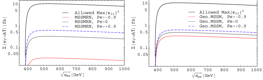
Fig. 1. – The production cross-section of e^- \gamma \rightarrow \tau^- A as a function of the center-of-mass energy \sqrt{s_{ee}} of the electron-electron system. Solid curve represents the result in the THDM with the maximal allowed value of |\kappa_{31}|^2 under the current experimental data in both figures.
