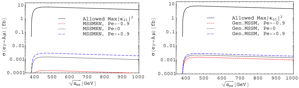
Fig. 2. – The production cross-section of e^- \gamma \rightarrow \mu^- A as a function of the center-of-mass energy \sqrt{s_{ee}} of the electron-electron system. Solid curve represents the result in the THDM with the maximal allowed value of |\kappa_{21}|^2 under the current experimental data in both figures.
