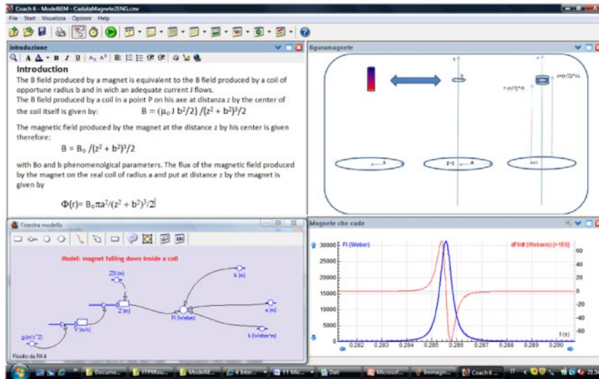
Fig. 5. – The model of the induced phenomena when a magnet is inserted into a coil: implementation in Coach 6 environment.
