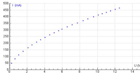
Fig. 2. – The I(U) characteristic of a bicycle bulb.
