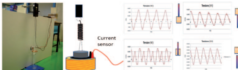
Fig. 4. – The experimental setup and exemplary data.
