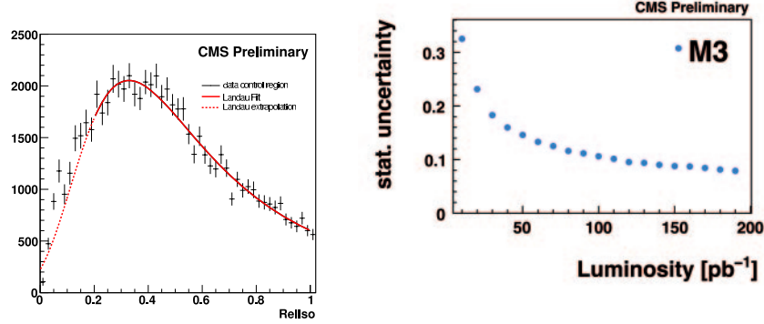
Fig. 2. – Left: fit with a Landau function to the RelIso distribution of events from a QCD dominated sample in the electron-plus-jets channel. The dashed line below 0.2 is an extrapolation. Right: expected statistical uncertainties as a function of the integrated luminosity.
