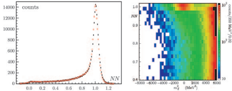
Fig. 1. – (Colour on-line) Left: neural-network output, NN , for electrons of a K_L \rightarrow \pi e \nu sample from data (black) and MC (red). Right: data density in the (NN, m_e^2) -plane: the signal is clearly visible at m_e^2 \sim 0 and NN \sim 1 .
