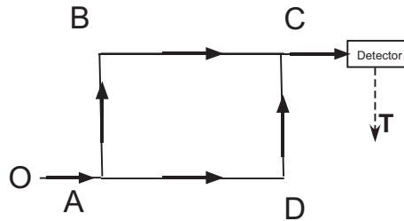
Fig. 1. – Diagram of an atom interferometer using the Mach-Zehnder concept.
