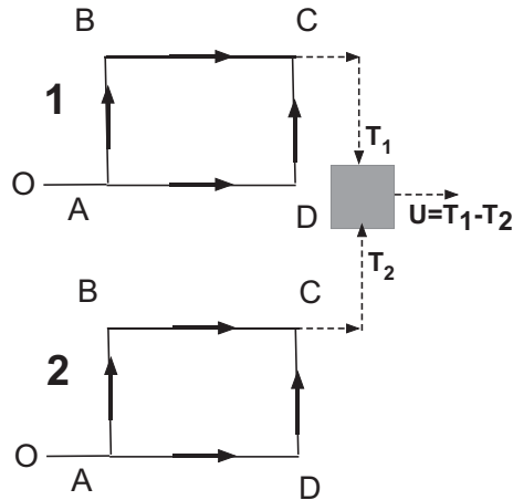
Fig. 2. – Diagram of the double atom interferometer.
