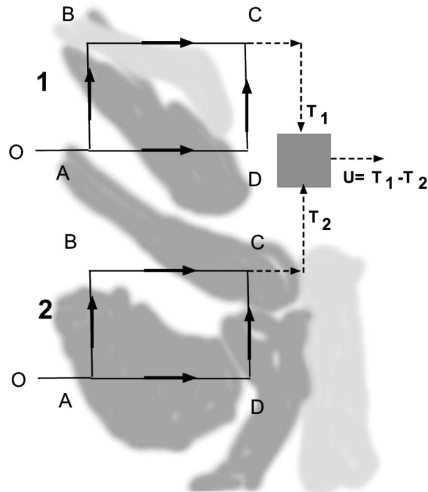
Fig. 3. – Illustration of how inhomogeneous dark energy density could produce a non-zero signal. The gray shapes represent the assumed inhomogeneity of the distribution of dark energy density.
