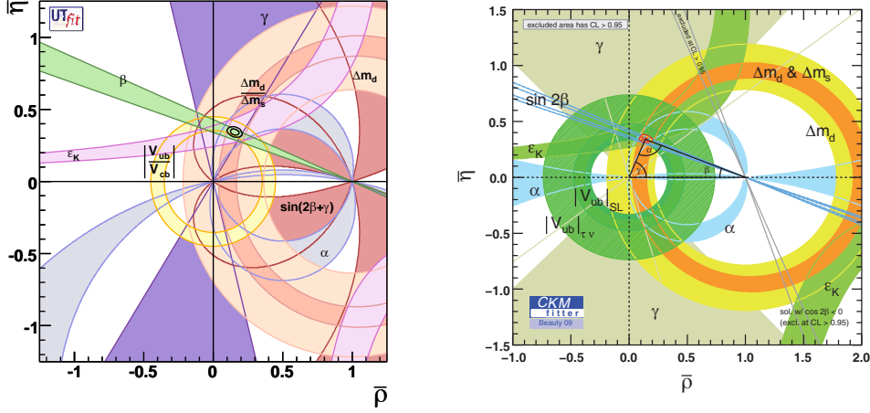
Fig. 1. – Constraints in the (\bar{\rho}, \bar{\eta}) -plane from a global CKM fit from UFit [1] (left plot) and CKMFitter [2] (right plot) Collaborations.
