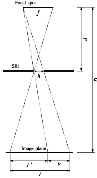
Fig. 1. – Typical geometrical setup for the focal-spot size measurement with the slit technique: focal-spot size ( f ), slit width ( h ), image size ( I ), penumbra ( p ) and focal-spot image ( f' ).
