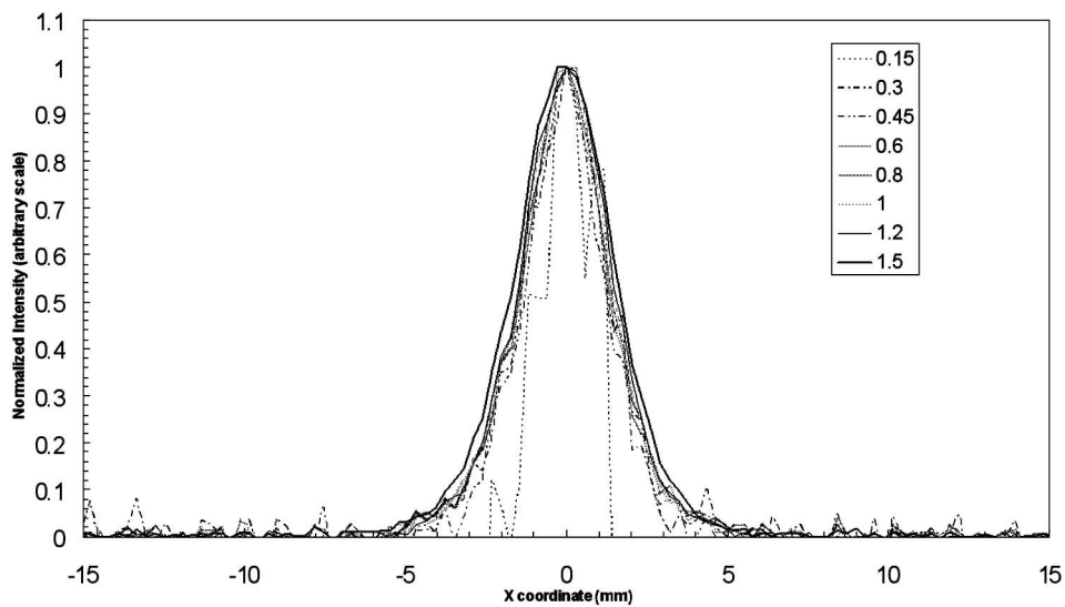
Fig. 6. – Plot of normalized image profiles obtained with a slit width ranging from 1.50 mm to 0.15 mm.
