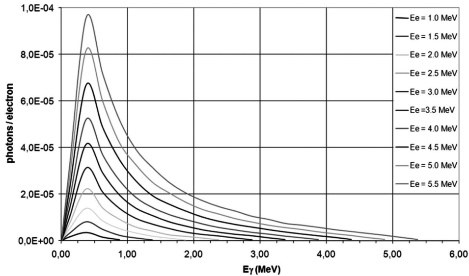
Fig. 2. – Bremsstrahlung spectra with different electron beam energy obtained with MC simulations.
