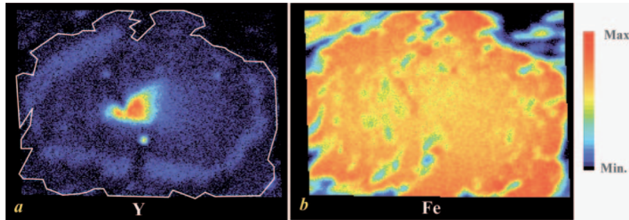
Fig. 4. – PIXE distribution maps of yttrium (a) and iron (b) in one of the analysed garnet crystals (the white line in (a) represents the crystal perimeter).
