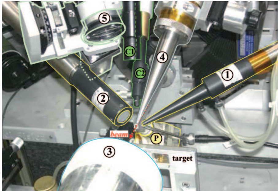
Fig. 3. – Beam end. (1) and (2): X-ray detectors optimized for low-medium- and medium-high-energy X-rays detection (PIXE); (3) \gamma -ray detector (PIGE); (4) vacuum-tight case containing the Si-photodiode for the detection of particles backscattered by the target (BS); (5) lens for light collection (IL); (P) Si-PIN detector for beam charge measure; (C1) and (C2) cameras for panoramic and microscopic sample visualization.
