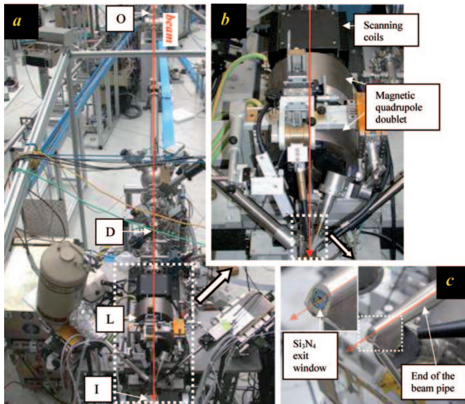
Fig. 2. – (a) General overview of the LABEC microbeam line, (b) strong focusing lens and scanning coils and (c) the end of the microbeam line with a blow-up on the beam extraction \text{Si}_3\text{N}_4 window (the dashed line rectangle indicates the part enlarged and shown in the following panel).
