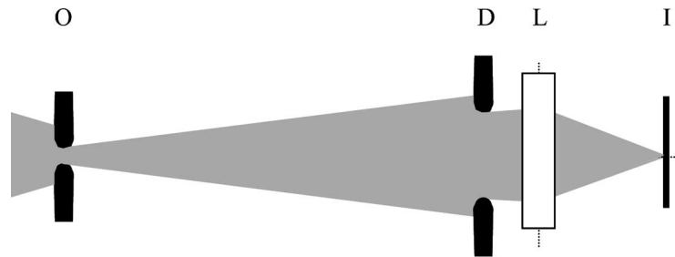
Fig. 1. – Scheme of a focusing system: L is a strong focusing lens which forms the image of the object O at the plane I. The diaphragm D controls the intensity of the beam arriving on the lens L and limits the aberrations introduced by L.
