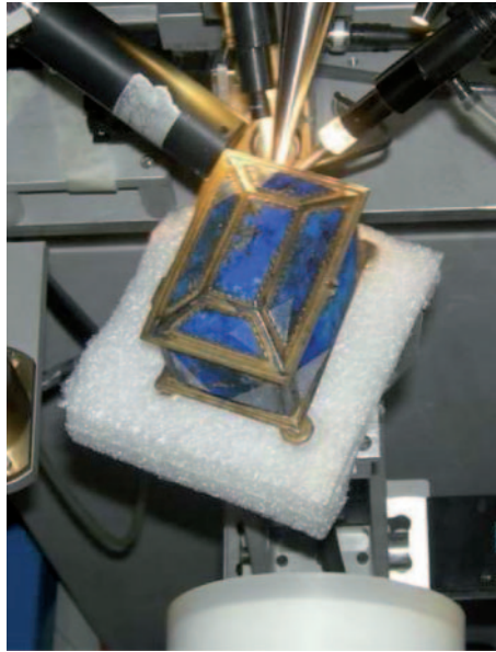
Fig. 5. – “Bauletto”, cat. N. [13684] from the “Collezione Medicea di Pietre Ornamentali”, Mineralogy and Lithology section of the Museum of Natural History, University of Florence, during the positioning for the analyses at the microbeam of LABEC.
