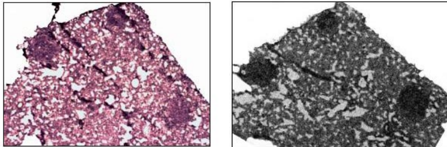
Fig. 1. – Comparison between the histological preparation of a lung section with tumor nodules (right) and the neutronigraphy of a subsequent section (left). The three circular darker structures on the left correspond to the three tumor nodules on the right, demonstrating that tumor cells uptake higher boron concentration with respect to normal tissue.
