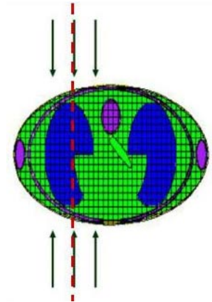
Fig. 3. – MCNP transversal view of ADAM's thorax, with the two ideal collimated epithermal beams for lung BNCT irradiation. The dashed line indicates the longitudinal axis of the lung, along which the uniformity of the thermal neutron field was studied.
