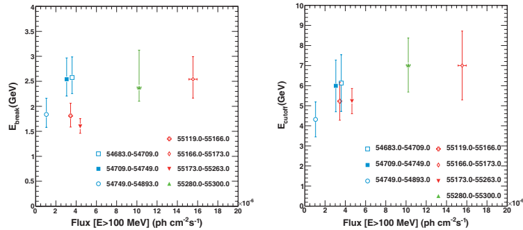
Fig. 3. – Evolution of E_{\text{break}} and E_{\text{cutoff}} with flux.
