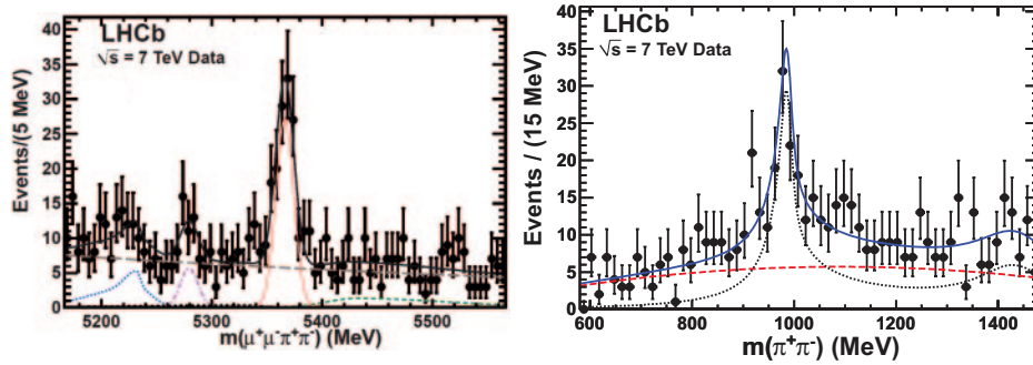
Fig. 10. – Left: The invariant mass of J/\psi\pi^+\pi^- combinations when the \pi^+\pi^- pair is required to be within \pm 90 MeV of the f_0(980) mass. The data have been fit with a signal Gaussian and several background functions. The thin (red) solid curve shows the signal, the long-dashed (brown) curve the combinatorial background, the dashed (green) curve the B^+ \rightarrow J/\psi K^+(\pi^+) background, the dotted (blue) curve the B^0 \rightarrow J/\psi K^{*0} background, the dash-dot curve (purple) the B^0 \rightarrow J/\psi\pi^+\pi^- background, the barely visible dotted curve (black) the sum of B_s^0 \rightarrow J/\psi\eta' and J/\psi\phi backgrounds, and the thick-solid (black) curve the total. Right: The invariant mass of \pi^+\pi^- combinations when the J/\psi\pi^+\pi^- combination is required to be within \pm 30 MeV of the B_s^0 mass. The dashed curve is the like-sign background that is taken from the data both in shape and absolute normalization. The dotted curve is the result of the fit described in [12].
