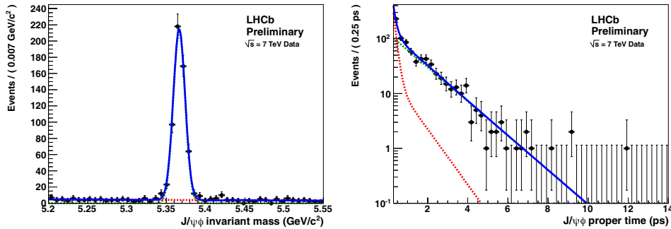
Fig. 4. – B_s^0 mass (left) and proper time (right) projections of the two-dimensional fit to the B_s^0 \rightarrow J/\psi\phi candidates with t > 0.3 ps. The total fit is represented by the blue solid line, the signal contribution by the green dashed line and the background contribution by the red dashed line. The mass range for the fit is m \in [5.20, 5.55] \text{GeV}/c^2 .
