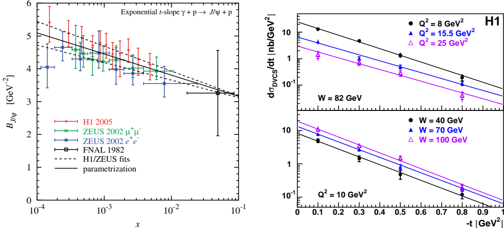
Fig. 3. – Left: dependence on x = M_V^2/W^2 of the slope parameter B_V of the exponentially falling |t| distributions for the exclusive production of J/\Psi mesons measured by the HERA collider experiments H1 and ZEUS and the FNAL E401/E458 experiments. The figure is taken from [10] with references for the data therein. Right: the DVCS cross-section differential in t for different values of Q^2 and W as indicated in the figure. The curves are results of fits of the form e^{-b|t|} . The figure is taken from [11].
