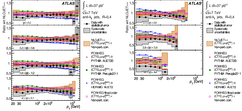
Fig. 5. – Ratio of measured inclusive jet cross section to next-to-leading-order calculation using NLOJet++ and the CT10 parton distribution functions (solid points). Different rapidity bins are shown and jets built with R = 0.4 are used. The shaded area around the data points represent the systematic uncertainty in the measurement. The hatched area around 1 represents the systematic uncertainty in the next-to-leading-order calculation. The other markers represent the next-to-leading-order calculation matched to parton showers implemented in POWHEG with different tunes and implementations [10].
