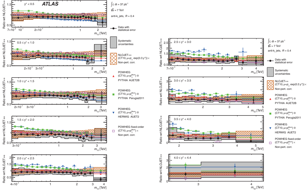
Fig. 6. – Ratio of measured dijet cross section to next-to-leading-order calculation using NLO-Jet++ and the CT10 parton distribution functions (solid points). Different y^* bins are shown and jets built with R = 0.4 are used. The different curves shown are as in fig. 5 [10].
