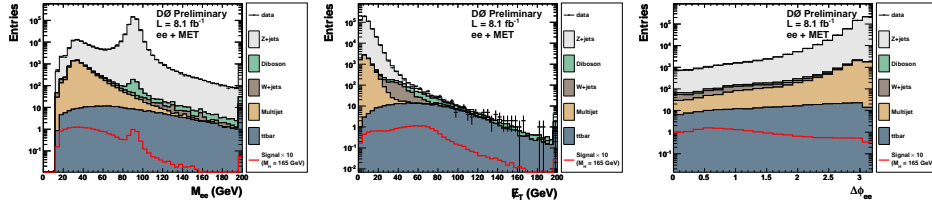
Fig. 1. – The invariant mass of isolated dileptons (left), the \cancel{E}_T spectrum of isolated leptons (center) and the \Delta\phi_{\ell\ell} for input to the discriminant analysis for the D0 experiment.
