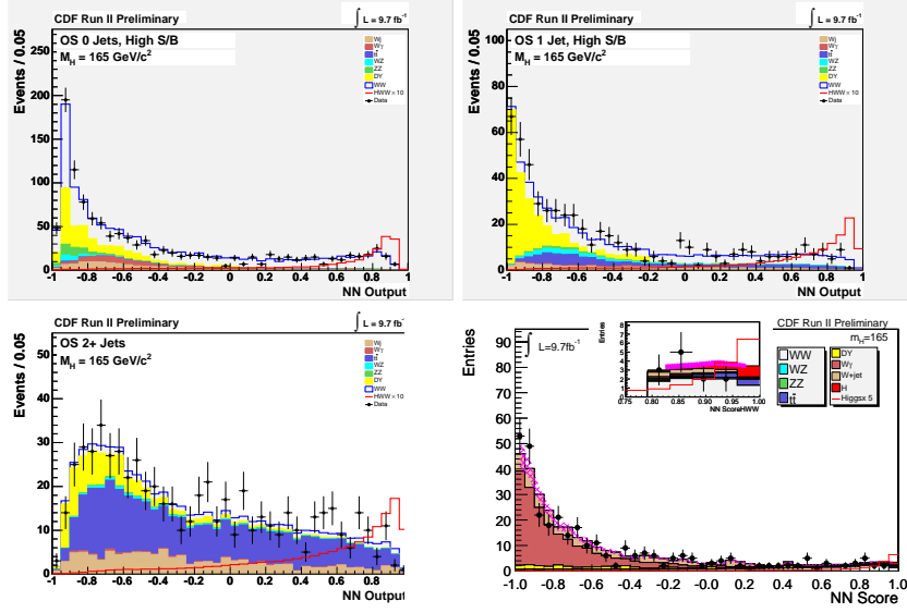
Fig. 2. – The Neural Net score distribution for opposite-sign dileptons in the 0, 1 and 2 jet for M_{\ell\ell} > 16 \text{ GeV}/c^2 and M_{\ell\ell} < 16 \text{ GeV}/c^2 channels.
