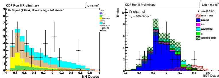
Fig. 3. – Neural net score distribution for for trileptons where opposite-sign pair invariant masses are in a 10 GeV window around the Z mass (left) and BDT distribution for the case where one of the trileptons is a hadronic tau (right).
