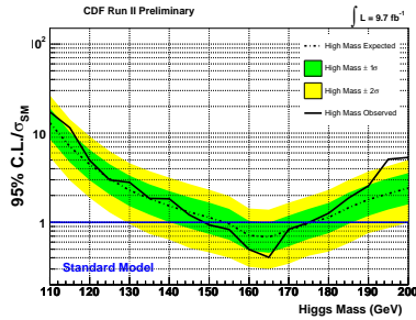
Fig. 4. – 95% confidence limits on the Standard Model Higgs boson for various masses for CDF for the 9.7\text{fb}^{-1} analysis.
