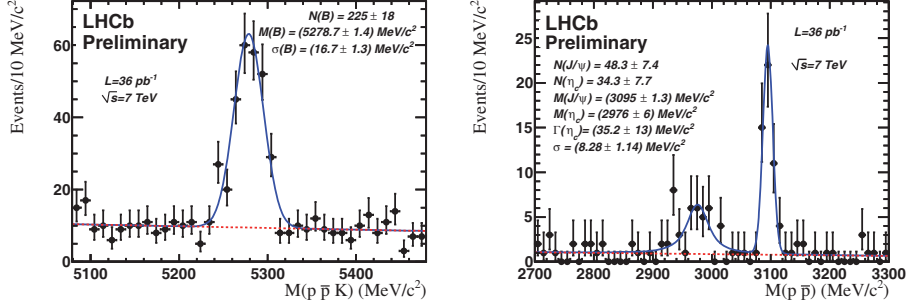
Fig. 1. – All B selected events (left) and p\bar{p} events (right).
