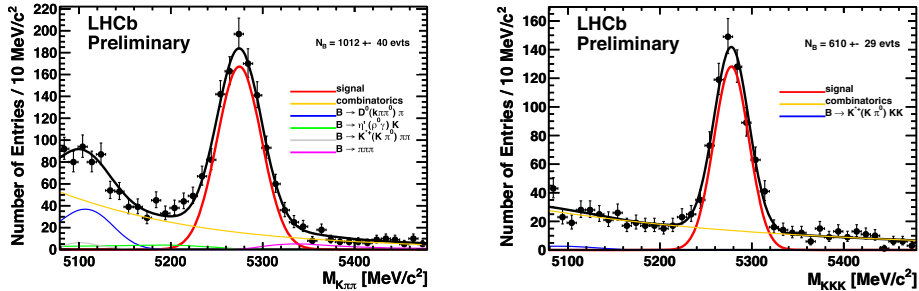
Fig. 2. – B^+ \rightarrow K^+\pi^+\pi^- (left) and B^+ \rightarrow K^+K^-K^+ (right) events.
