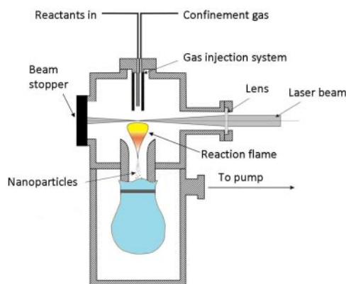
Fig. 1. – Scheme of the set-up for laser synthesis of nanoparticles from gas phase reactants.
