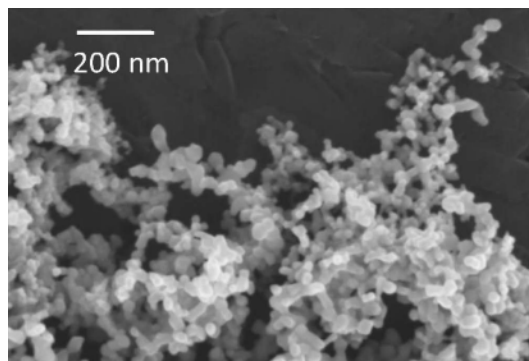
Fig. 4. – SEM image of \text{TiO}_2 nanoparticles produced by \text{CO}_2 laser pyrolysis of TTIP, after annealing in air to remove the contaminants.
