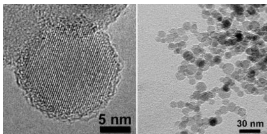
Fig. 3. – TEM images of Si nanoparticles produced by \text{CO}_2 laser pyrolysis of silane. Courtesy of Prof. G. Mattei and Dr. V. Bello, University of Padua, Italy [8].
