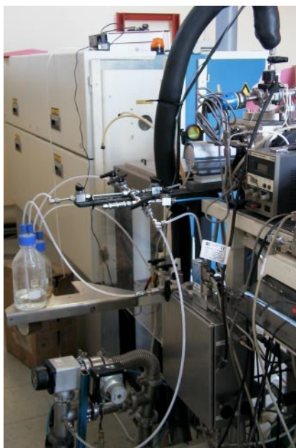
Fig. 2. – Picture of the gas injection system for use of liquid precursors in the laser pyrolysis set-up.
