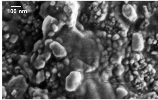
Fig. 6. – High-magnification SEM image of grey Carrara marble treated with Paraloid B72/TiO 2 (0.2% w/v): the nanoparticles induces a micro- and nano-scale roughness at the acrylic surface. Courtesy of L. Pilloni, ENEA.
