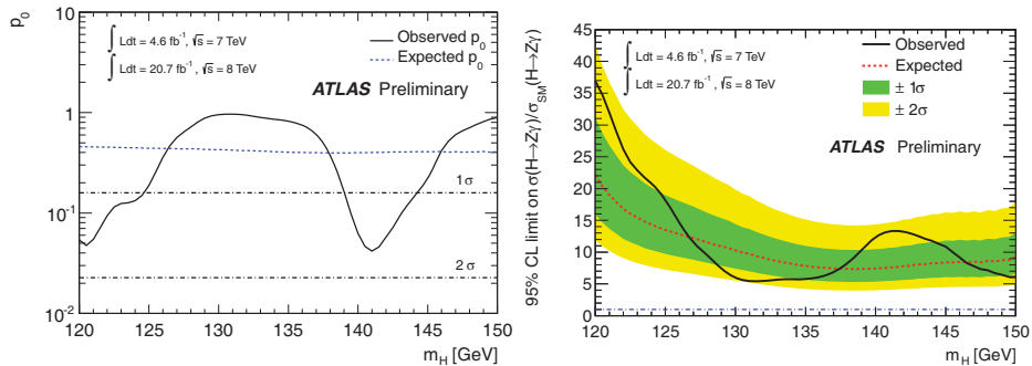
Fig. 3. – Left: expected (dashed blue line) and observed (solid black line) p_0 (compatibility of the data with the background-only hypothesis) as a function of the Higgs boson mass, using 4.6\text{ fb}^{-1} of pp collisions at \sqrt{s} = 7\text{ TeV} and 20.7\text{ fb}^{-1} of pp collisions at \sqrt{s} = 8\text{ TeV} . Right: observed 95% CL limits (solid black line) on the production cross section of a SM Higgs boson decaying to Z\gamma , as a function of the Higgs boson mass. The median expected 95% CL exclusion limits (dashed red line) are also shown. The green and yellow bands correspond to the \pm 1\sigma and \pm 2\sigma intervals.
