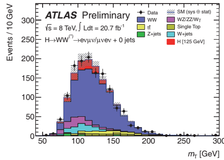
Fig. 1. – m_T distribution for the 0 jet DF channel [1].
