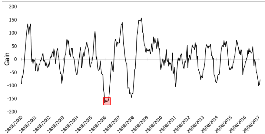
Fig. 2 An example of the Local Gain value Time Series (LGTS) of a generic OP pixel. The moment when LGTS is minimum (red) is assumed as the moment of the forest loss (intermediate date between the beginning and the completion of forest cut)
