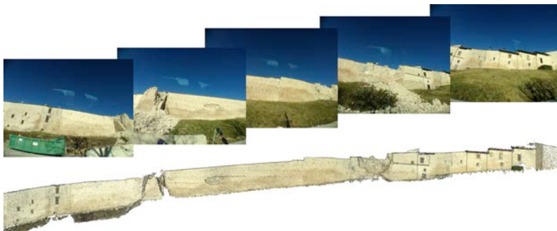
Fig. 2 Frames of Norcia's image sequence and 3D point cloud frontal view
