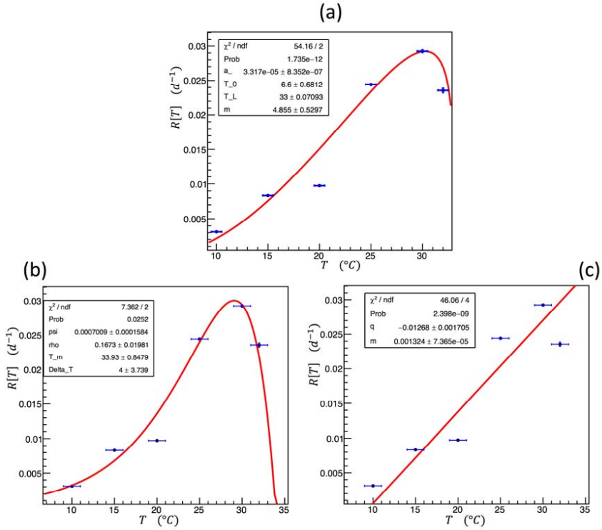
Fig. 1 Graphical fit results from fitfisso.c macro with data related to L. botrana (Moshtagi Maleki et al., 2016). The best fit parameters are reported in Tab. 1. (a) is the Briere rate function, (b) is the Logan rate function and (c) is the linear fit function
