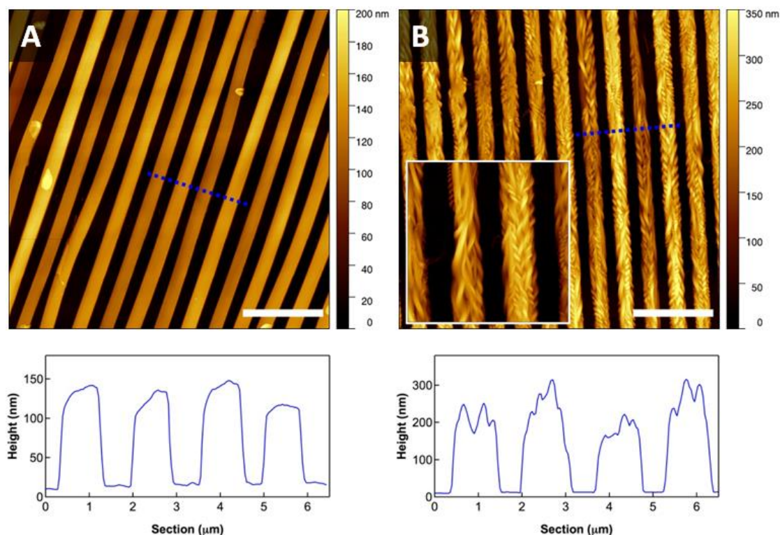
Figure 2. AFM images 20 \times 20 \mu\text{m}^2 and related height plots of the fibers of: (A) 2 and (B) 4 patterned according the Lithographically Controlled Wetting (LCW) 21 technique. Scale bars = 5 \mu\text{m} . Inset image (B): zoom 5 \times 5 \mu\text{m}^2 .
