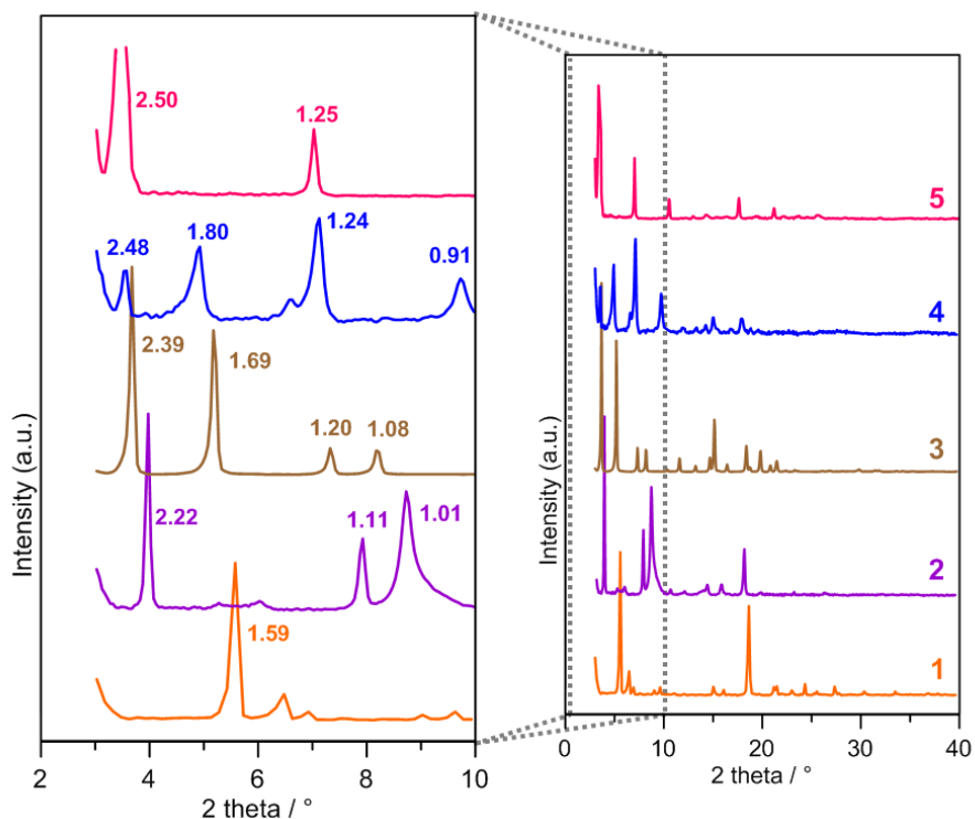
Figure 6. X-ray diffraction pattern of the fibers of 1-5 grown on glass.
