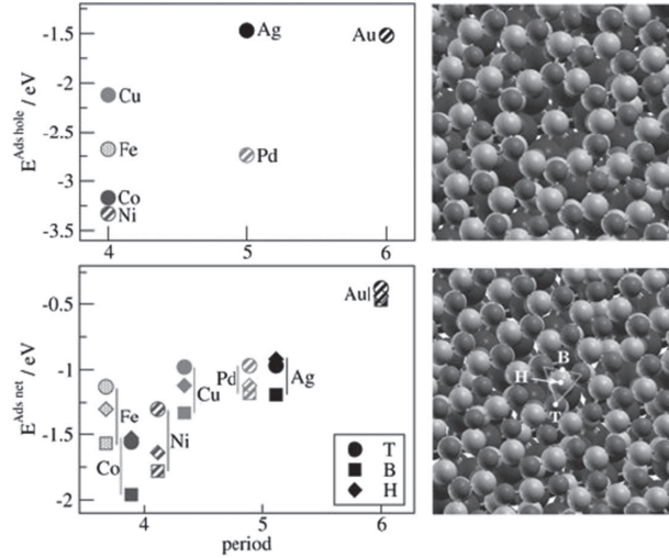
Fig. 3. – Left panels: DFT adsorption energies of several transition metal atoms in the “hole” of the alumina film (upper panel) and in three inequivalent sites (hollow (H), bridge (B), top (T)) close to the three-fold “network” position (lower panel). Right: top view of the corresponding structural models of the alumina film around the adsorption sites. Small medium grey balls: O atoms; small light grey: Al; small dark grey: Ni.
