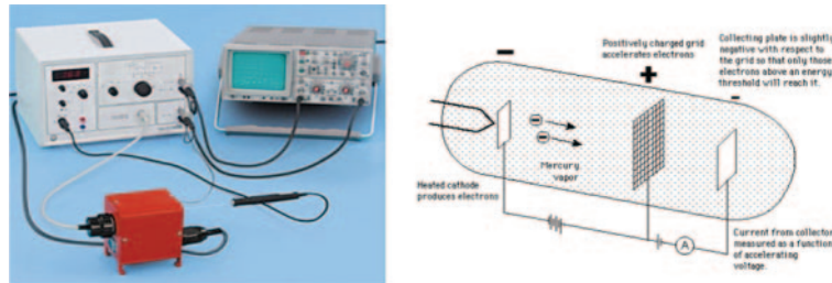
Fig. 1. – Experimental set-up for the Franck-Hertz experiment (left) and schematic representation of the mercury-filled Franck-Hertz tube (right).
