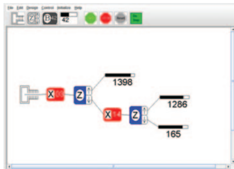
Fig. 5. – Spins Stern-Gerlach simulation.
