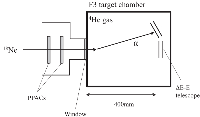
Fig. 1. – The schematic experimental setup is shown. A 3.6 \text{ MeV/u } ^{18}\text{Ne} beam was bombarded on the ^4\text{He} gas target. Scattered \alpha particles were detected by silicon detector telescopes. Two PPACs located just before the target chamber provide beam current and position information.
