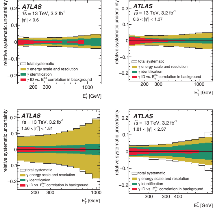
Fig. 1. – Total relative systematic uncertainty in [1], excluding that in the luminosity measurement, as a function of E_T^\gamma for different regions of \eta^\gamma as well as the contributions from the photon energy scale and resolution (yellow histogram), the photon identification (green histogram) and the photon identification vs. E_T^{\text{iso}} correlation in the background (red histogram). The histograms show the stacked contributions.
