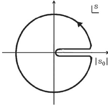
Fig. 1. – The squared energy s -plane used in Cauchy's theorem, eqs. (1), (2).
