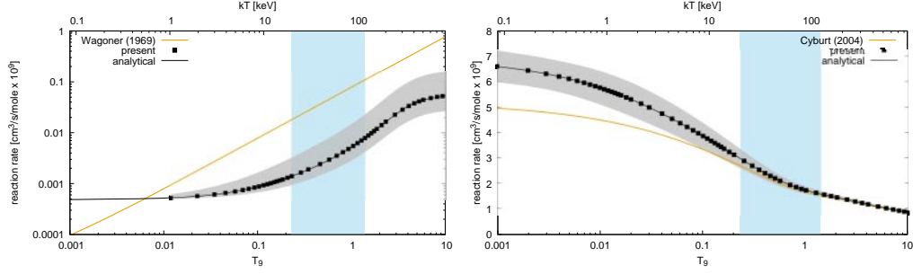
Fig. 1. – Reaction rates N_A\langle\sigma v\rangle for the {}^7\text{Be}(n, \alpha){}^4\text{He} (left) and {}^7\text{Be}(n, p){}^7\text{Li} (right), shown in comparison to rates used before the n_TOF measurements. The gray bands around the analytical curves indicate the evaluated uncertainties on the rates, while the vertical band indicates the temperature of interest in BBN network calculations.
