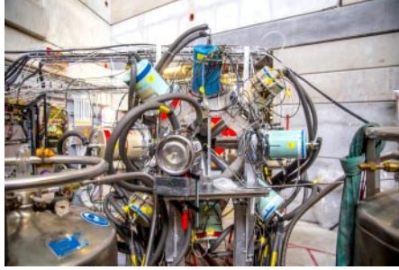
Fig. 1. – Setup for the test of muon transfer reactions in a high-density-deuterium gas mixture at the \pi E1 area at PSI. The gas target is placed at the center of the detector array.
