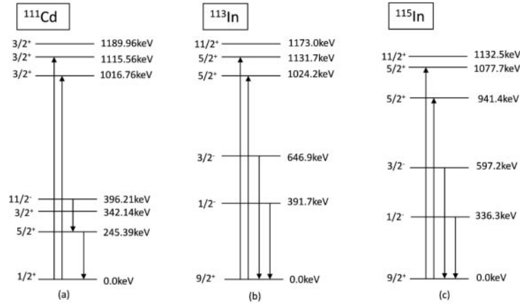
Fig. 1. – Energy level diagram of the excited states of (a) ^{111}\text{Cd} at 1016.76 keV, (b) ^{113}\text{In} at 1024.2 keV, and (c) ^{115}\text{In} at 941.4 keV [4].
