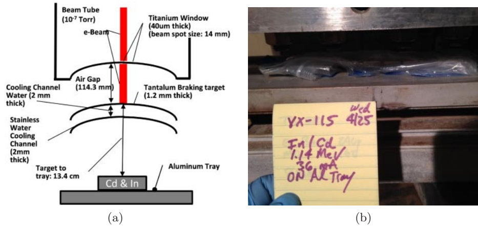
Fig. 3. – View of Cd and In sample location under the beam. (a) Cross sectional view of electron beam, titanium window, braking target, cooling channel, and sample location and (b) photograph of Cd and In sample on the aluminum product tray.
