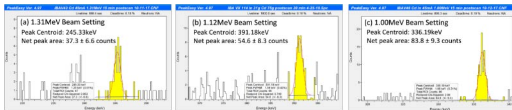
Fig. 4. – Gamma scans of Cd and In samples with background subtracted. (a) ^{111m}\text{Cd} : 1.31 MeV beam energy (15min scan), (b) ^{113m}\text{In} : 1.12 MeV beam energy (30min scan), (c) ^{115m}\text{In} : 1.00 MeV beam energy (15 min scan).
