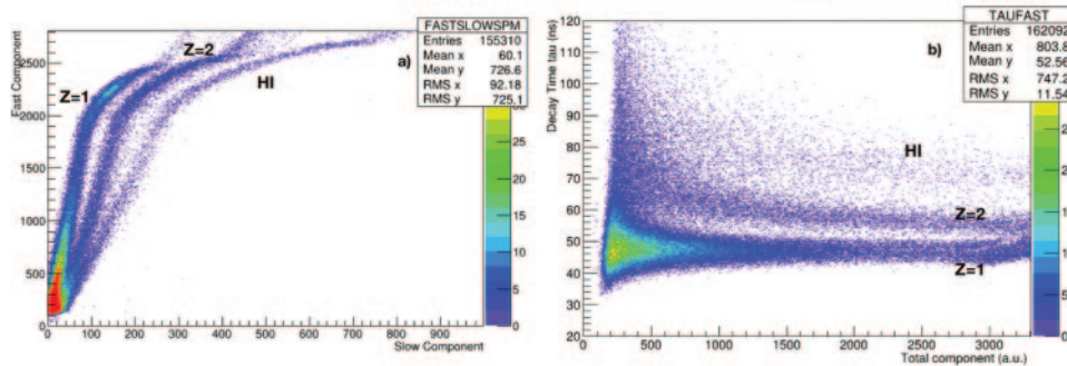
Fig. 8. – EJ276 coupled with a silicon photomultiplier (i-SPECTOR). (a) Fast vs. slow component 2D identification matrix. (b) Decay time vs. total energy (for more detail see [10]).
