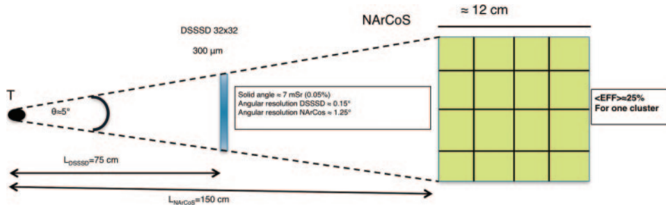
Fig. 1. – Schematic view of the NArCoS prototype coupled with the DSSSD. Possible distances from the target positions are indicated [14-16].
