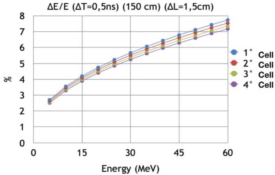
Fig. 2. – Predicted energy resolution for neutrons from the TOF technique. Each line represents one of the four elementary cells of a cluster (see text), the considered time resolution (500 ps) follows the assumption to use a fast detector as start of the TOF ( e.g. , a MCP).
