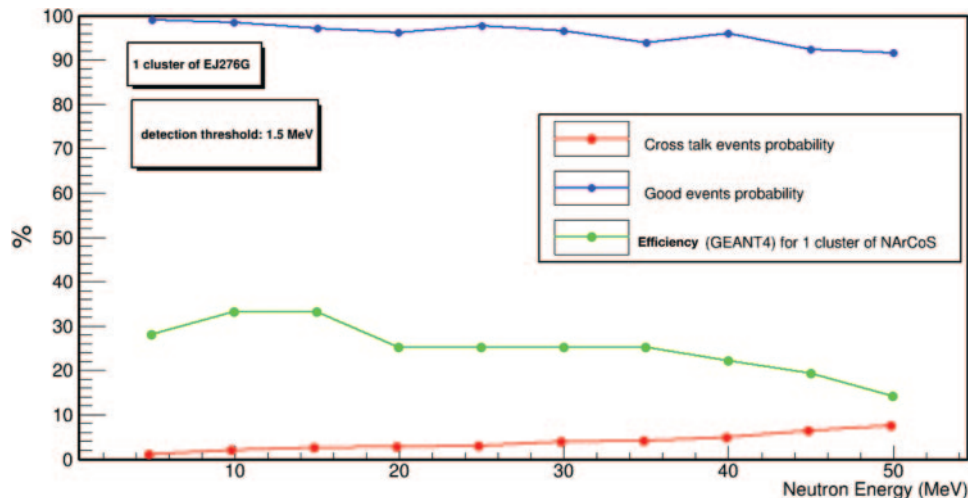
Fig. 6. – GEANT4 simulated cross-talk probability (red line), good events probability (blue line) and efficiency (green line) for detail see text.
