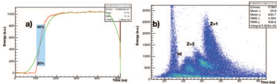
Fig. 7. – EJ276G coupled with a silicon photodiode. (a) Example of a digitalized signal with GET electronic [34]. (b) Plastic+SiPD PSD discrimination, total energy vs. signal rise time.
