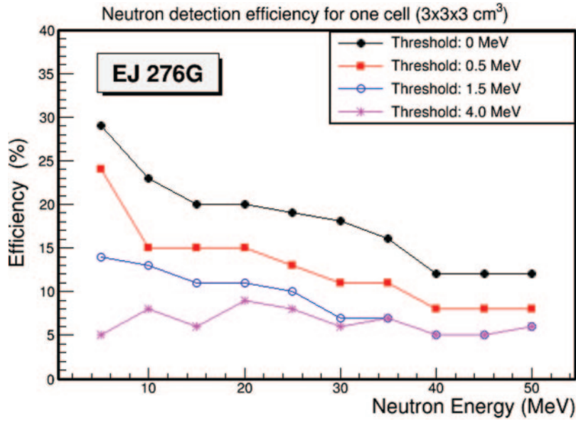
Fig. 4. – GEANT4 [17,18] efficiency simulations for one elementary cell. The lines represent different considered threshold values [15,16].
