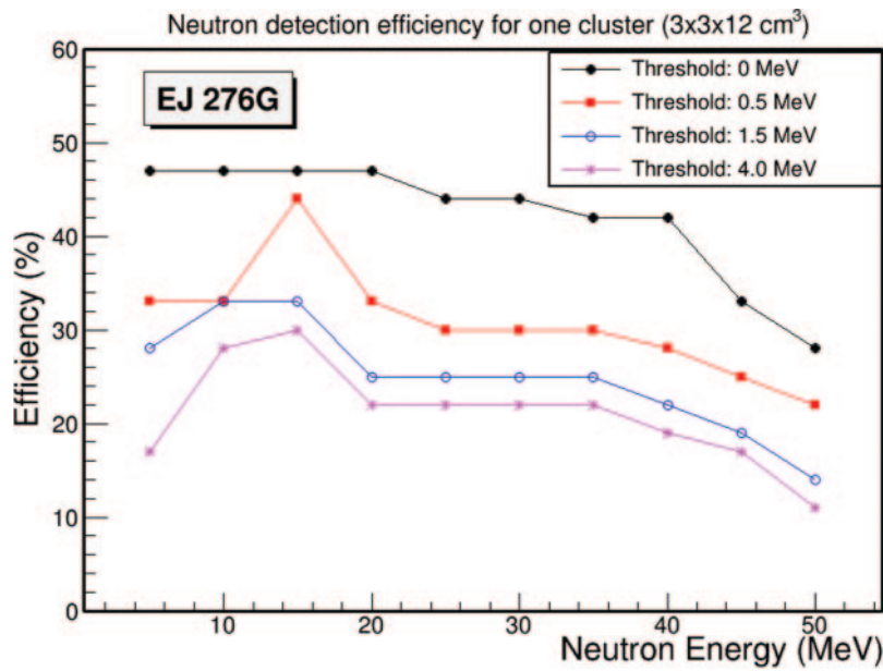
Fig. 5. – GEANT4 [17,18] efficiency simulations for one cluster. The lines represent different considered threshold values [15,16].
