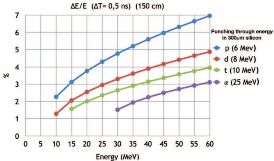
Fig. 3. – Predicted energy resolution for light charged particles from the TOF technique, the considered time resolution (500 ps) follows the assumption to use a fast detector as start of the TOF ( e.g. , a MCP).
