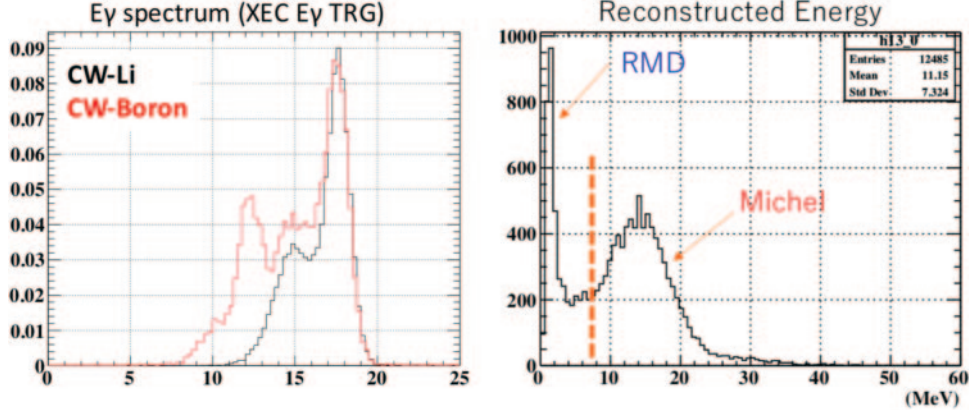
Fig. 7. – Left: photon energy spectrum used to calibrate LXe. Right: positron reconstructed energy from RDC.
