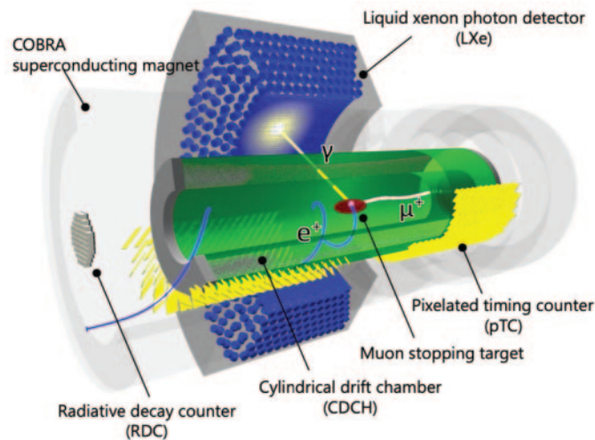
Fig. 1. – Experimental layout of the MEG II experiment.
