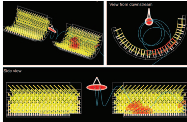
Fig. 5. – Schematic views of the pTC modules.
