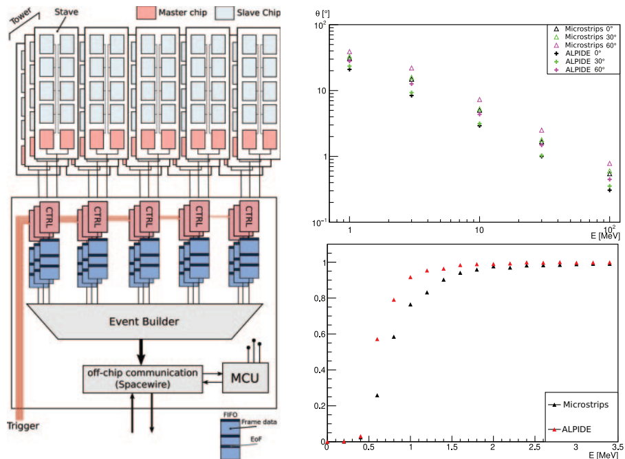
Fig. 1. – (Left) Tracker and readout system architecture. (Right) Simulation of energy threshold and angular resolution for incident electrons.
