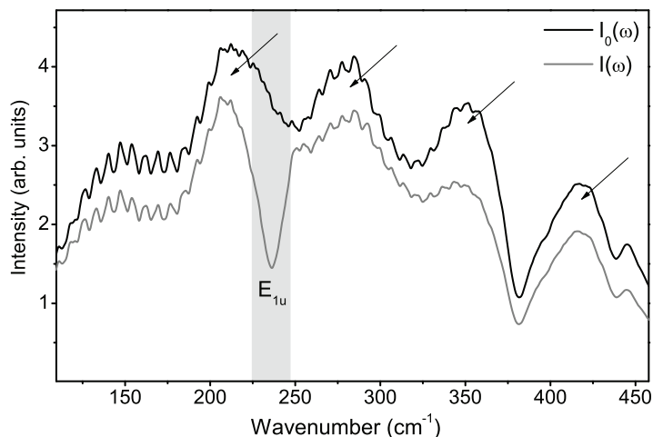
Fig. 2. – Background intensity ( I_0(\hat{\nu}) ) and transmitted intensity ( I(\hat{\nu}) ) at 1 GPa. Black arrows indicate the large interference fringes in the two spectra. Grey rectangle highlights the E_{1u} peak in the transmitted intensity.
