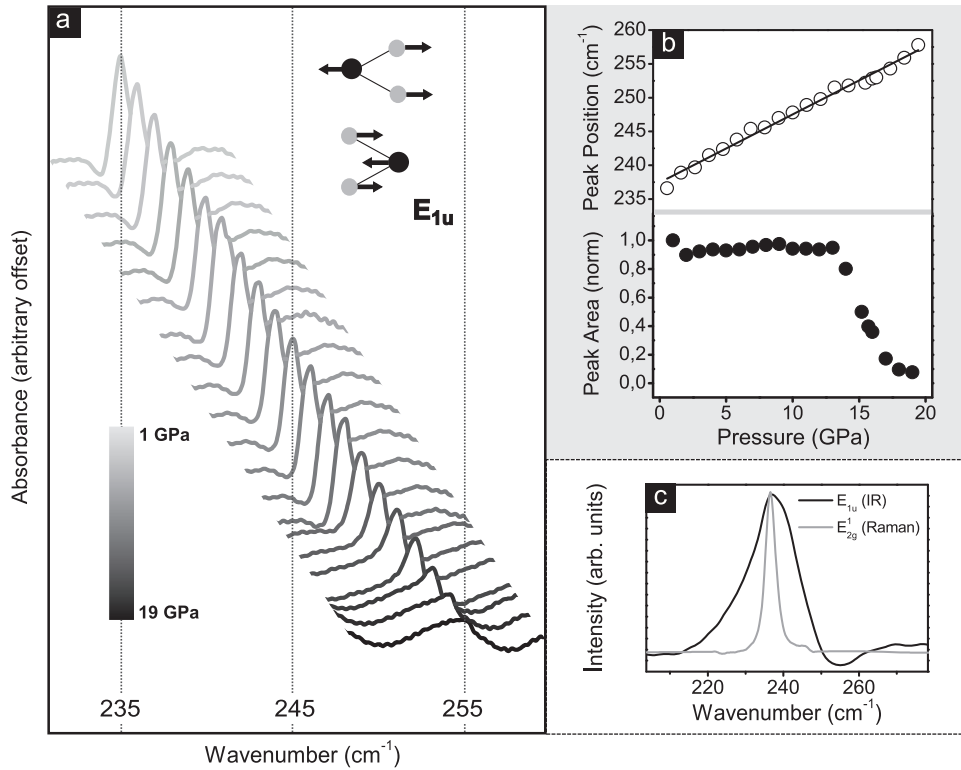
Fig. 3. – (a) Absorbance spectra in the frequency region around the E_{1u} peak; offsets have been arbitrary shifted to highlight the peak evolution under pressure. (b) On the top, peak position as a function of the pressure; the solid line represents the linear fit of the experimental data. On the bottom, peak area as a function of the pressure normalized to the 1 GPa value. (c) Line-shapes of IR-active E_{1u} , in black, and Raman-active E_{2g}^1 , in red, at 2 GPa; the intensities have been rescaled to ease the comparison between the two peak profiles.
